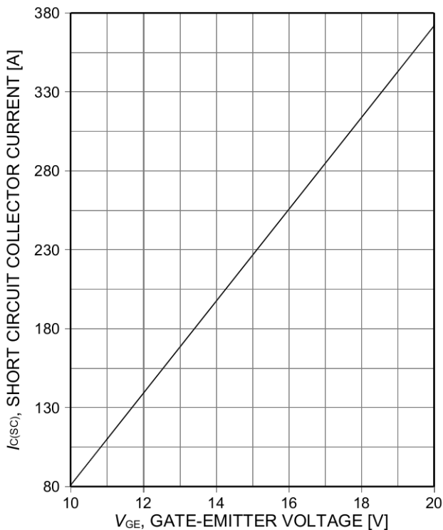
Figure 19. Typical short circuit collector current as a function of gate-emitter voltage ( V_{CE} \le 400V , start at T_j=25^\circ C )
