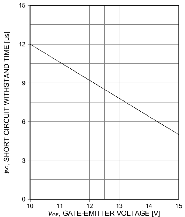
Figure 20. Short circuit withstand time as a function of gate-emitter voltage ( V_{CE} \le 400V , start at T_j \le 150^\circ C )
