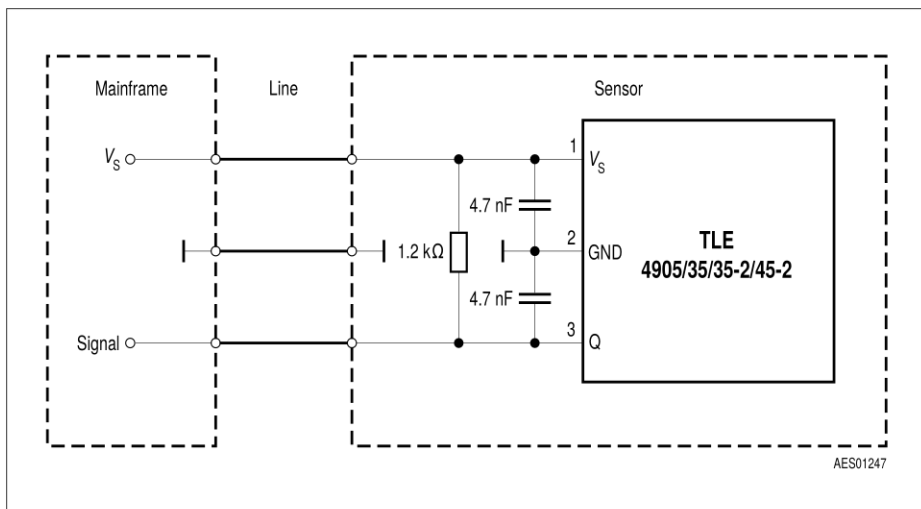
Figure 8 Application Circuit
