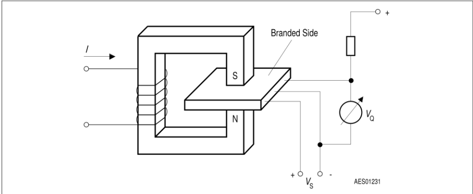
Figure 3 Sensor/Magnetic-Field Configuration
