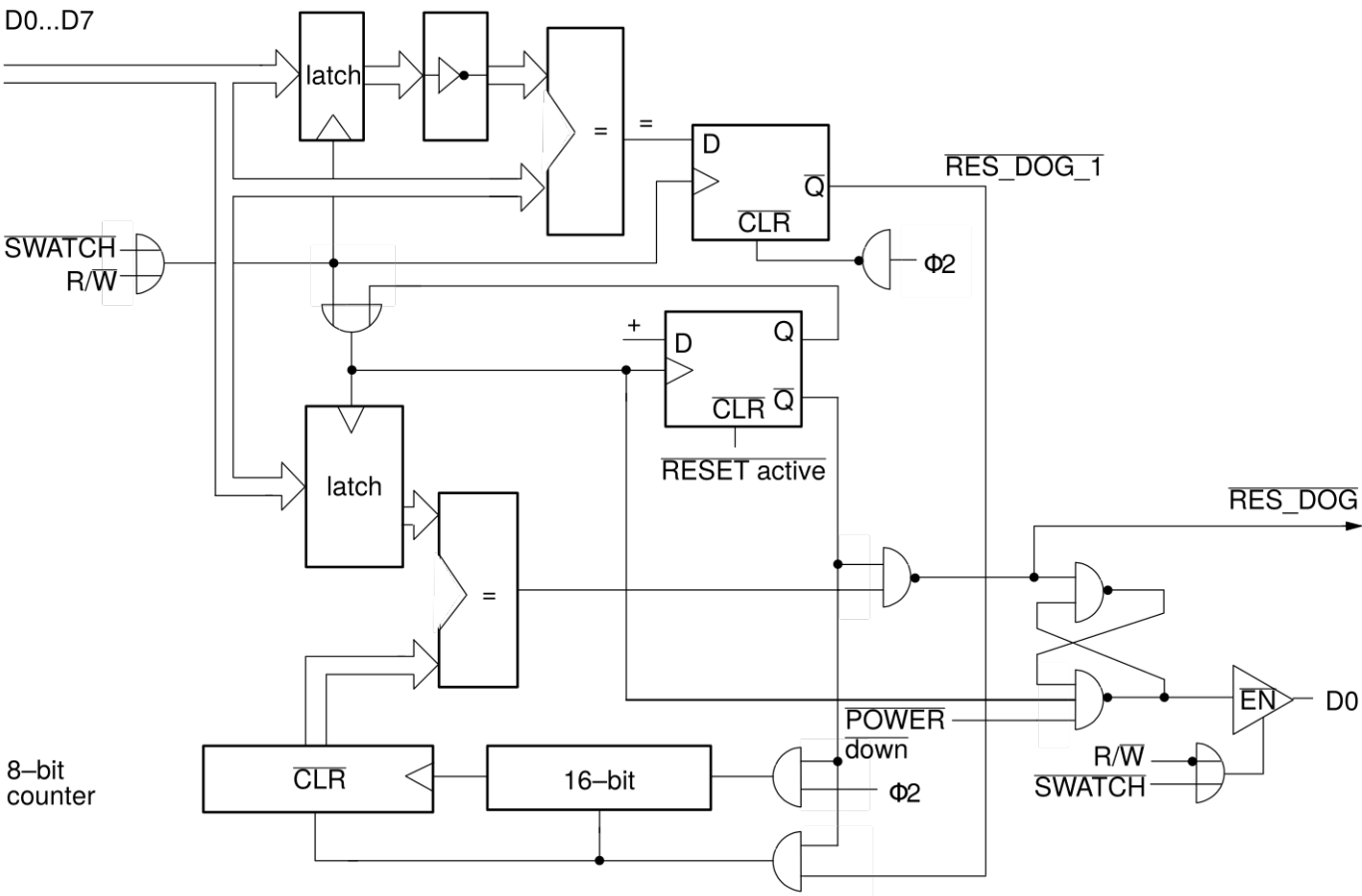
Fig. 2-17: Watchdog
