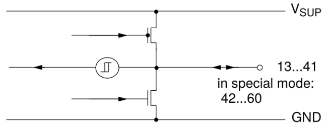
Fig. 4-10: P1, P2, P3, Timer (1, 2, 3), IR (Input only), in special mode: P5, P7, P8
