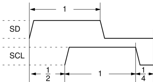
Fig. 2-20: Start condition I²C bus
