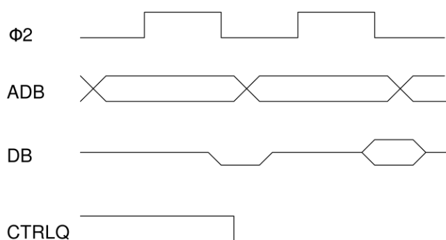
Fig. 2-10: Static control signals interrupt Bits 2, 3
