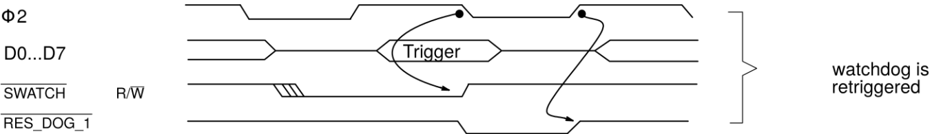
Fig. 2-18: Timing watchdog
