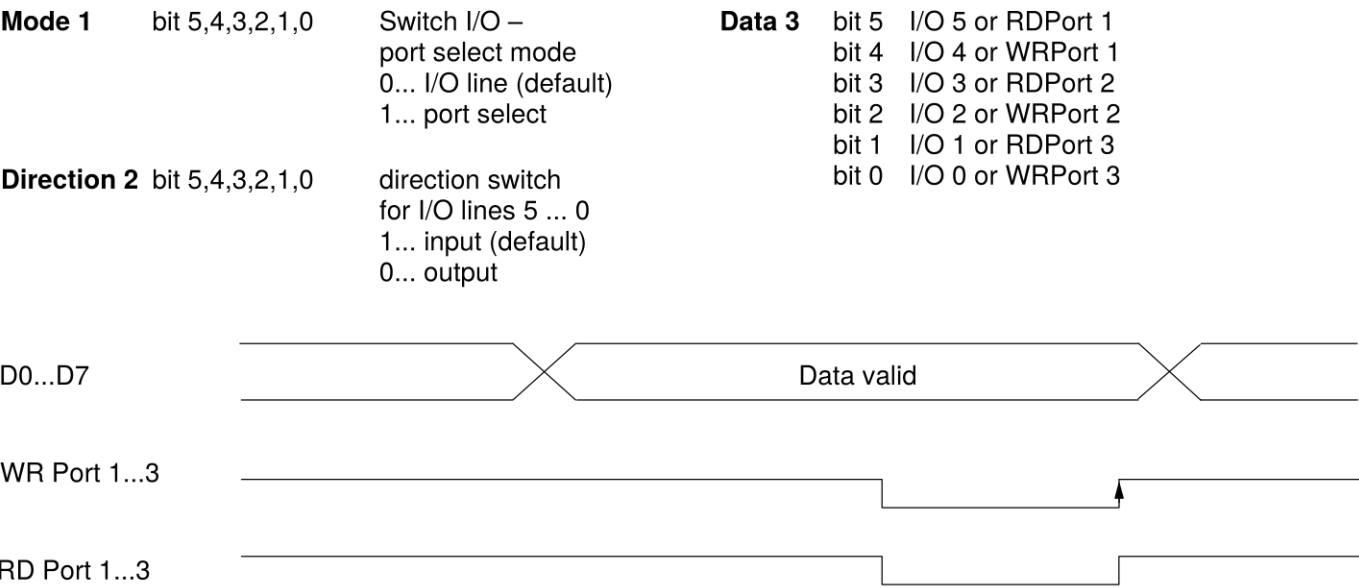
Fig. 2–1: Timing diagram
