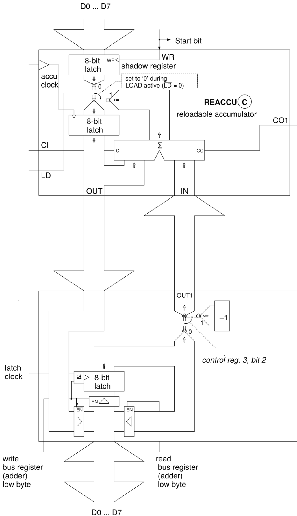
Fig. 2-14: Reloadable accumulator
