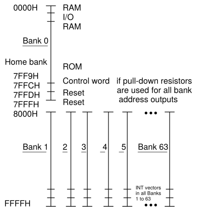
Fig. 2-4: Memory Map, up to 2 MByte
