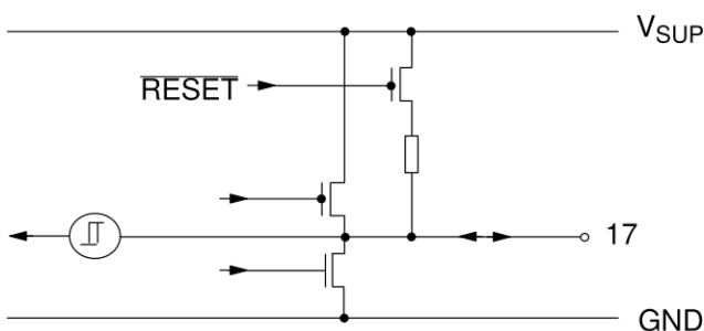
Fig. 4-9: R/W, CCU 3000
