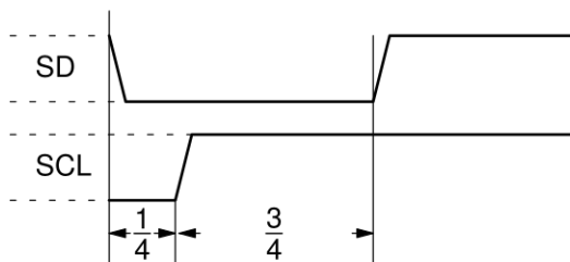
Fig. 2-22: Stop condition I²C bus
