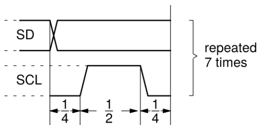
Fig. 2-21: Single bit on I²C bus
