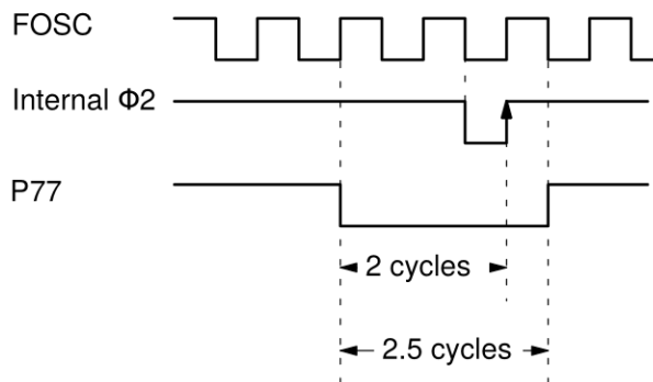
Fig. 2-3: Power-down control
