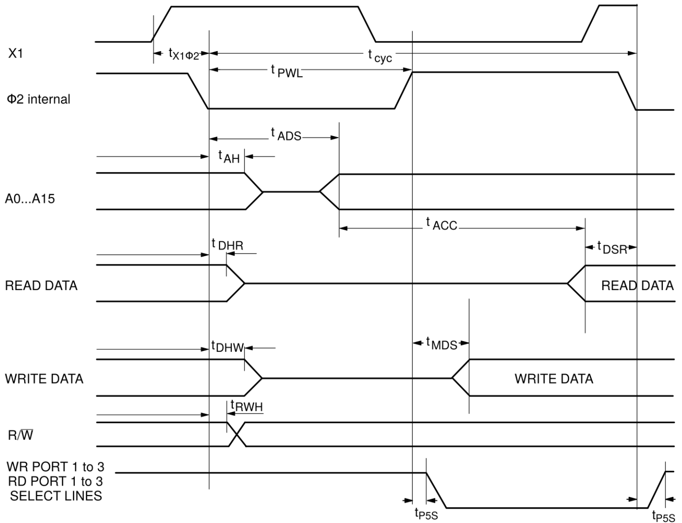
Fig. 4-13: AC timing
