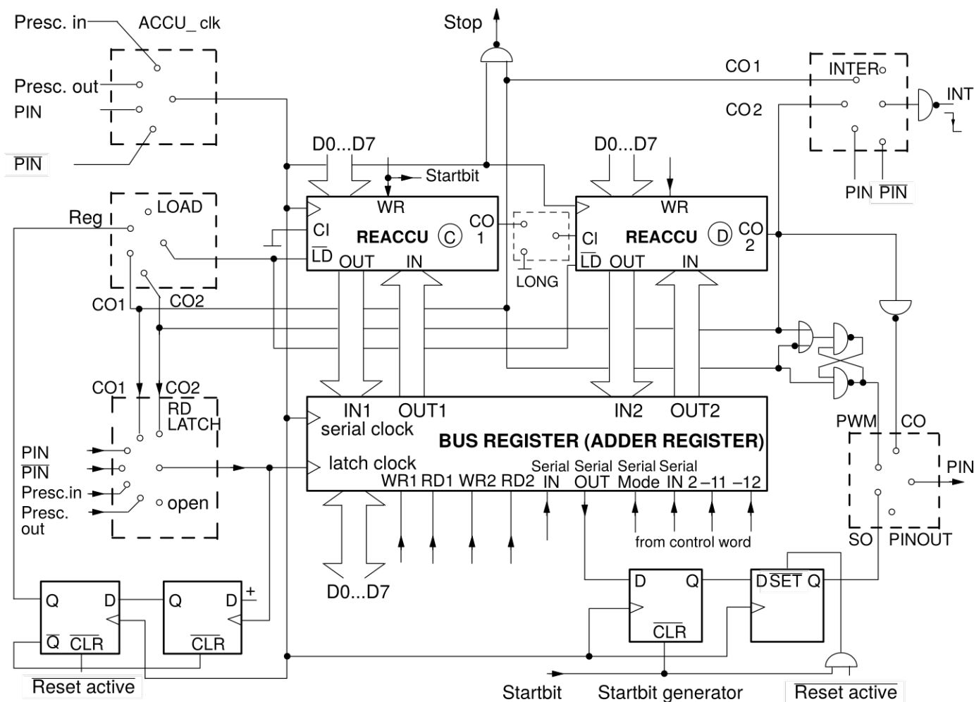
Fig. 2-16: Timer
