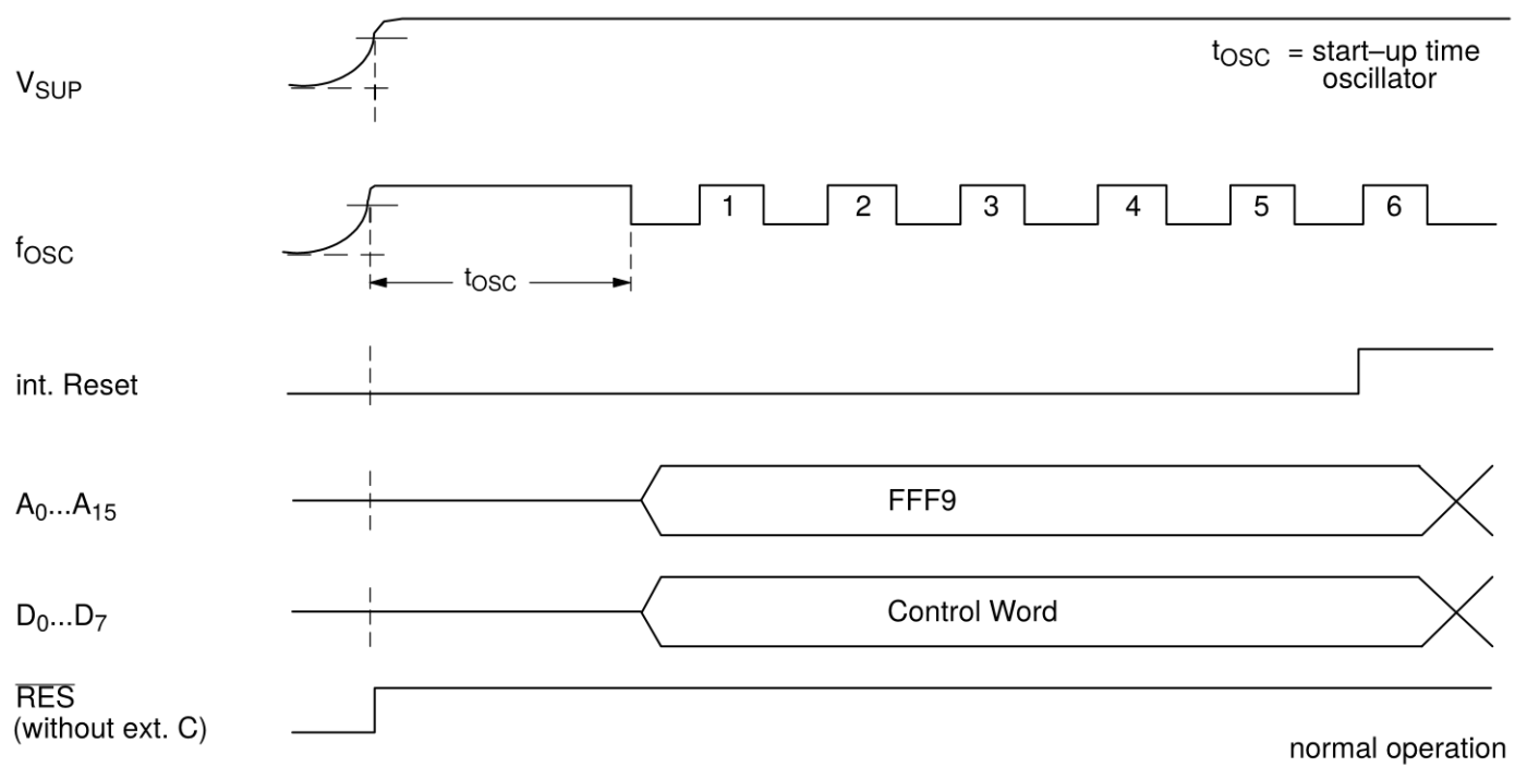
Fig. 2-7: Power-on sequence
