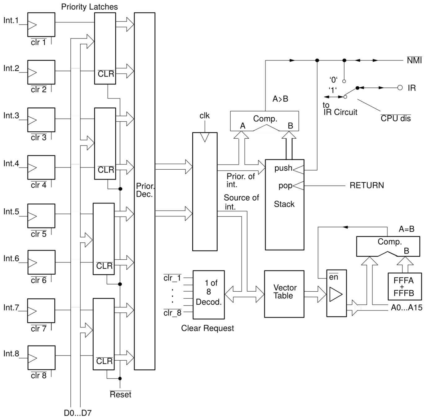
Fig. 2-11: Interrupt controller
