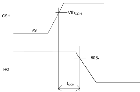
Figure 3: V_S > V_{th_{OCL}} to Shutdown Waveform
