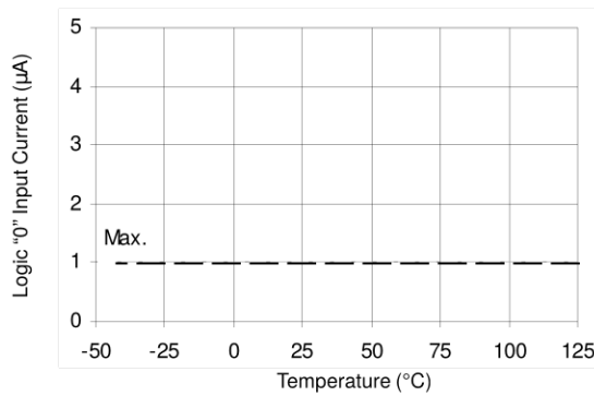
Figure 20A. Logic "0" Input Current vs Temperature
