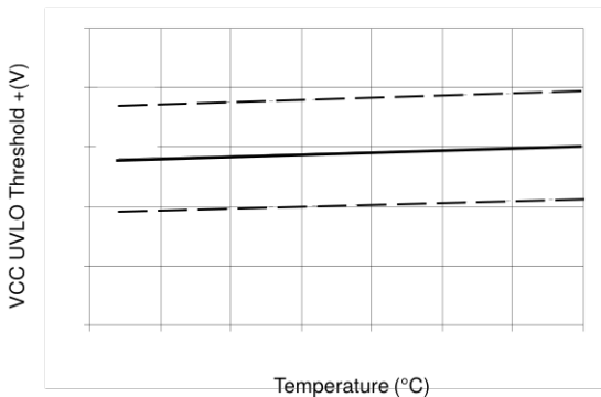
Figure 21A. Vcc Undervoltage Threshold(+) vs Temperature
