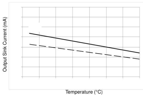
Figure 23A. Output Sink Current vs Temperature
