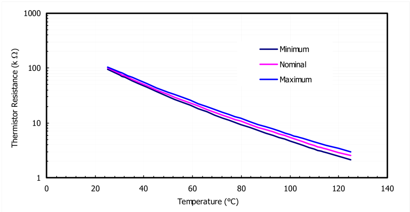
Figure 7. Variation of thermistor resistance with temperature
