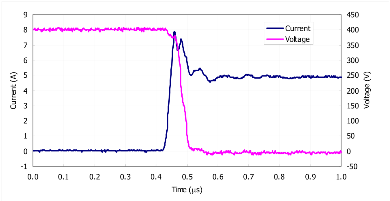
Figure 5. IGBT Turn-on. Typical turn-on waveform @ T_j=125^{\circ}\text{C} , V_{\text{BUS}}=400\text{V}
