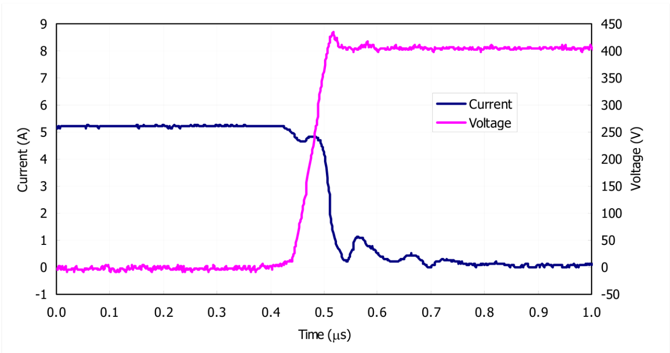
Figure 6. IGBT Turn-off. Typical turn-off waveform @ T_j=125^{\circ}\text{C} , V_{\text{BUS}}=400\text{V}
