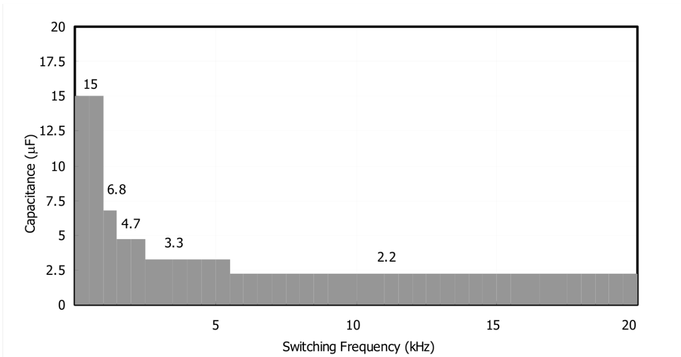
Figure 10. Recommended minimum Bootstrap Capacitor value Vs Switching Frequency
