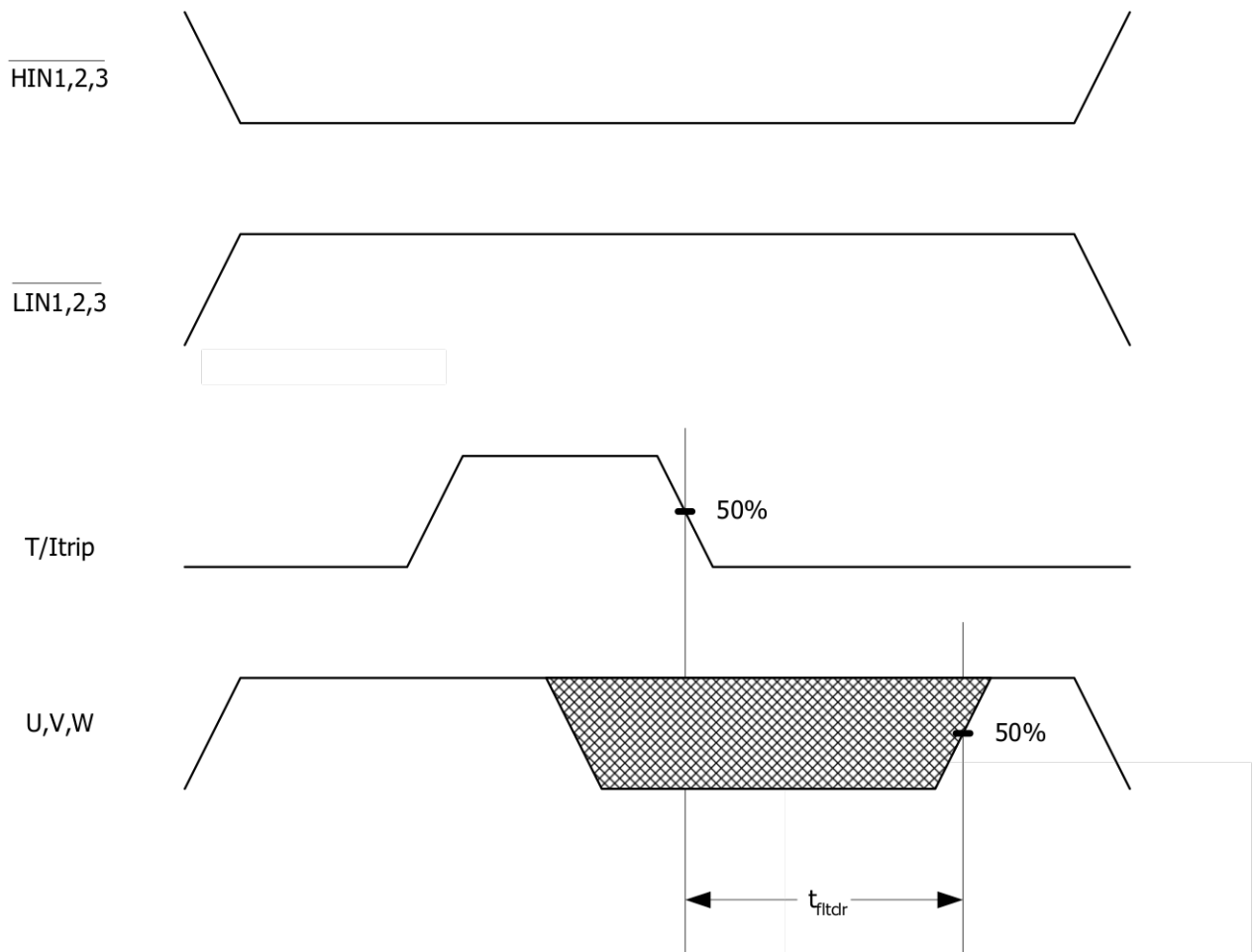
Figure 2. T/I_{Trip} Timing Waveform
