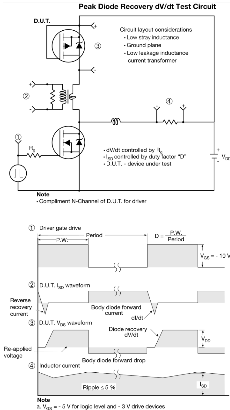
Fig. 14 - For P-Channel
