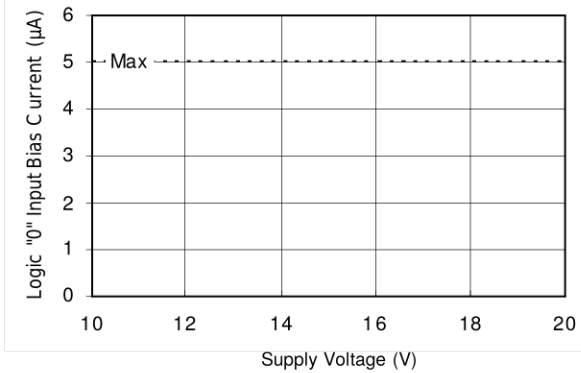
Figure 20B. Logic "0" Input Bias Current vs. Voltage
