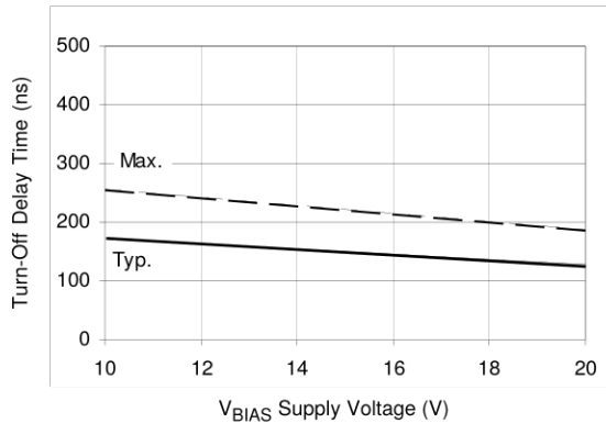
Figure 7B. Turn-Off Time vs. Supply Voltage
