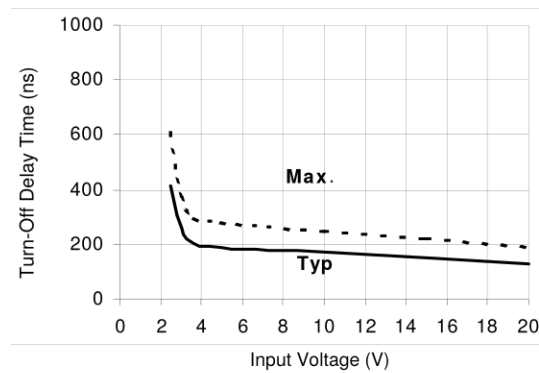
Figure 7C. Turn-Off Time vs. Input Voltage
