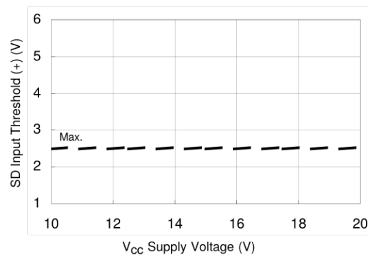
Figure 24B. SD Input Positive Going Threshold (+) vs. Supply Voltage
