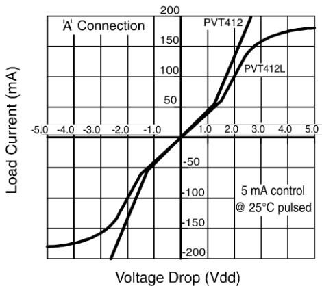
Figure 3. Linearity Characteristics
