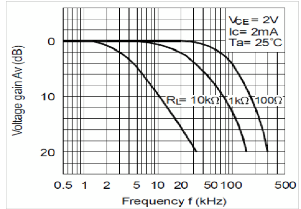
Fig 8 Frequency Response
