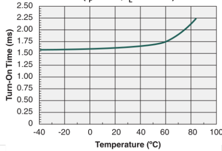
Typical Turn-On Time vs. Temperature ( I_F=3mA, I_L=100mA )
