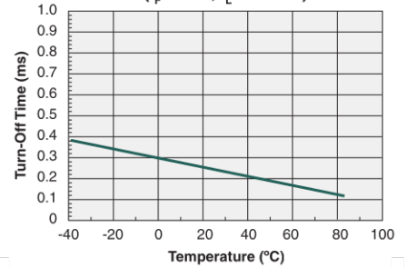
Typical Turn-Off Time vs. Temperature ( I_F=3mA, I_L=100mA )
