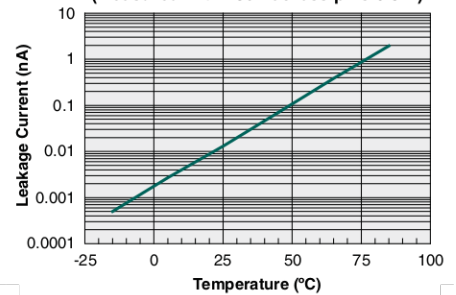
Typical Leakage Current vs. Temperature (Measured with 250V across pins 6 & 4)
