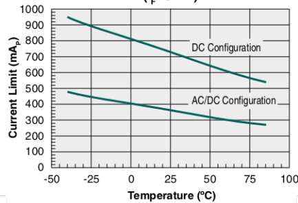
Typical Current Limit vs. Temperature ( I_F=5mA )
