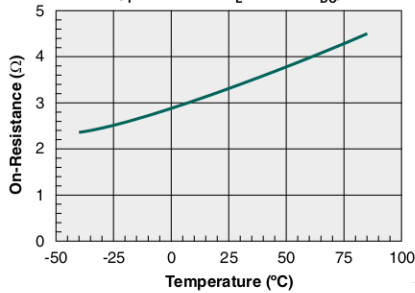
On-Resistance vs. Temperature DC-Only Configuration ( I_F=2-10mA , I_L=100mA_{DC} )
