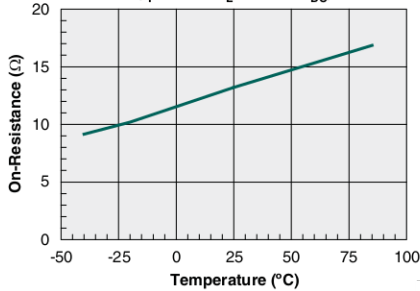
On-Resistance vs. Temperature DC-Only Configuration ( I_F=2-10mA , I_L=100mA_{DC} )
