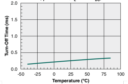
Typical Turn-Off Time vs. Temperature ( I_F=2-10mA , I_L=10mA_{DC} )
