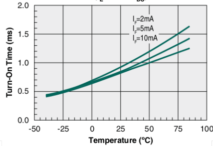
Typical Turn-On Time vs. Temperature ( I_L=10mA_{DC} )
