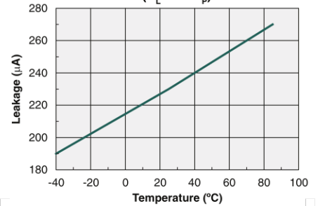
Typical Leakage vs. Temperature (V L =600V P )
