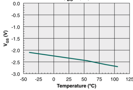
Threshold Voltage ( I_D=1\mu A )
