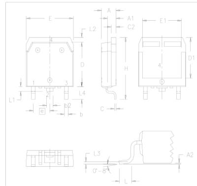
TO-268 (IXFT) Outline
