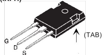
TO-268 (IXFT)
