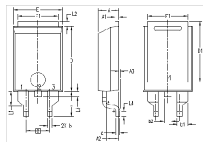
PLUS220SMD (IXFV_S) Outline
