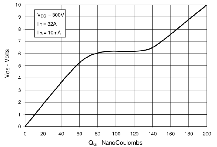
Fig. 7. Gate Charge
