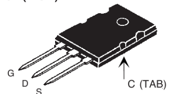
TO-264 (IXGK)
