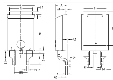
PLUS220SMD (IXTV_S) Outline
