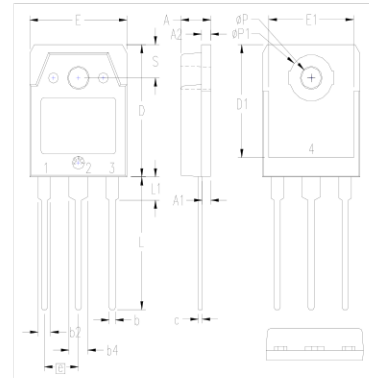
TO-3P (IXTQ) Outline
