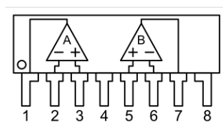
SIP8 Package
