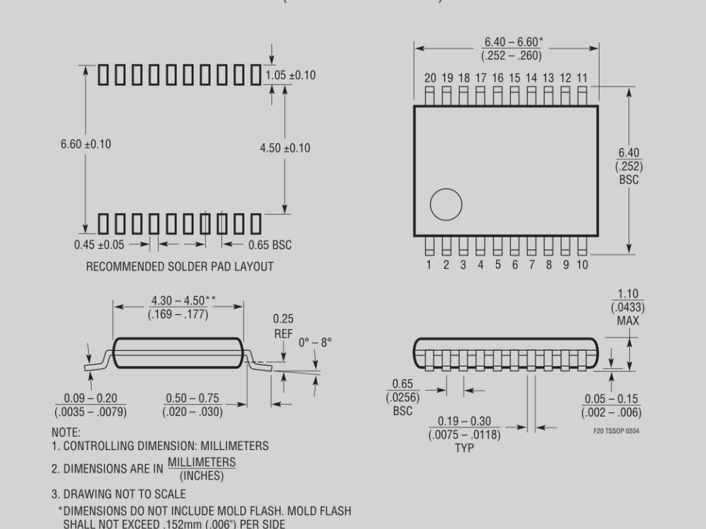
F Package 20-Lead Plastic TSSOP (4.4mm) (LTC DWG # 05-08-1650)
