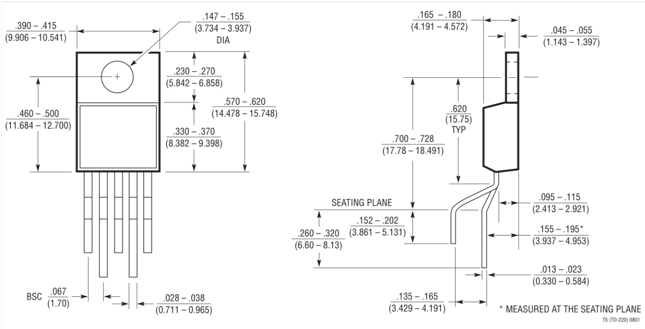
T Package 5-Lead Plastic TO-220 (Standard) (LTC DWG # 05-08-1421)
