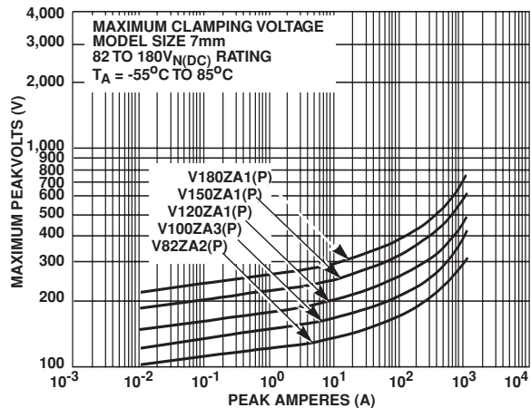
FIGURE 7. CLAMPING VOLTAGE FOR V82ZA2(P) - V180ZA1(P)
