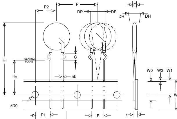
Crimped Leads "ZT"
