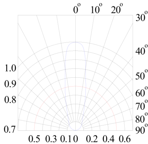
Radiation Diagram
