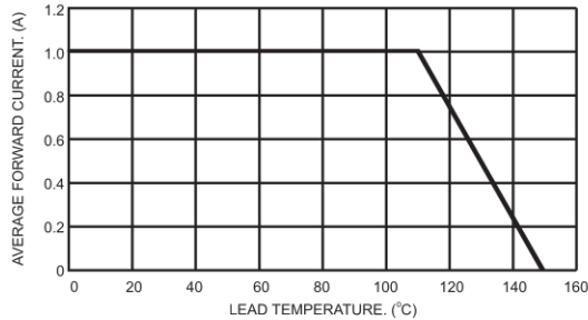
FIG.1- MAXIMUM FORWARD CURRENT DERATING CURVE
