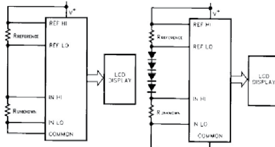
ICL7106 system setup for 2V reference ICL7106 system setup for 200mV reference Figure 22. Ratimetric Ohms Measurement
