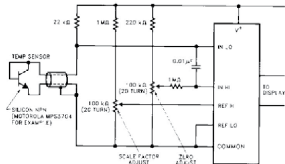
Figure 20. Digital Thermometer
