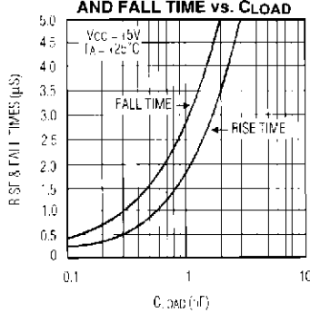
MAX620/MAX621 DRIVER RISE AND FALL TIME vs. LOAD
