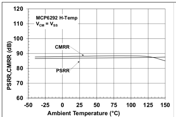
FIGURE 2-37: MCP6292 H-Temp CMRR, PSRR vs. Ambient Temperature.
