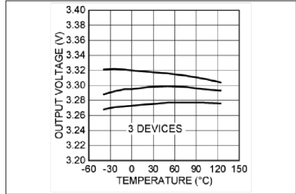
FIGURE 2-53: MIC29500-3.3 Output Voltage vs. Temperature.
