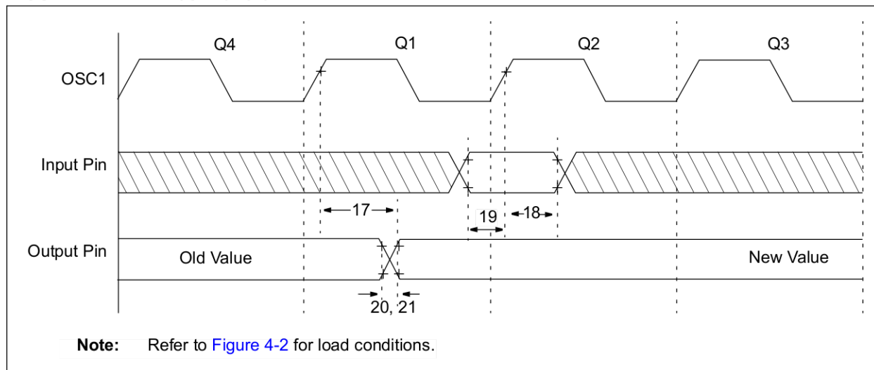
FIGURE 4-4: I/O Waveform
