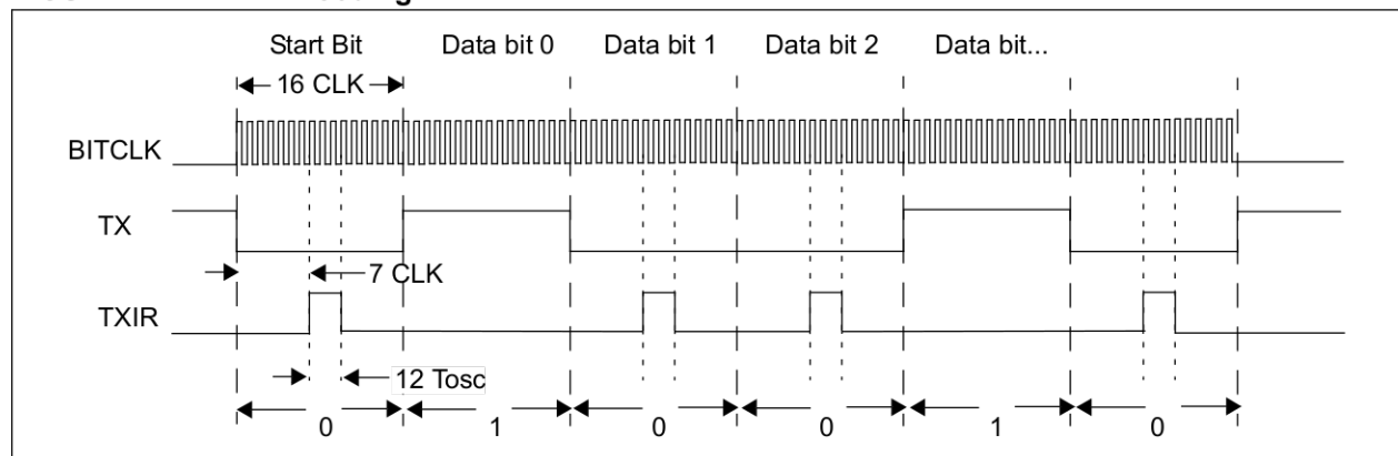
FIGURE 2-2: Encoding
