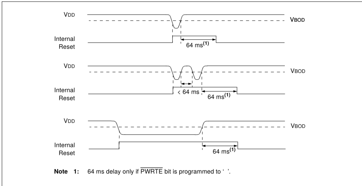
FIGURE 12-3: BROWN-OUT SITUATIONS
