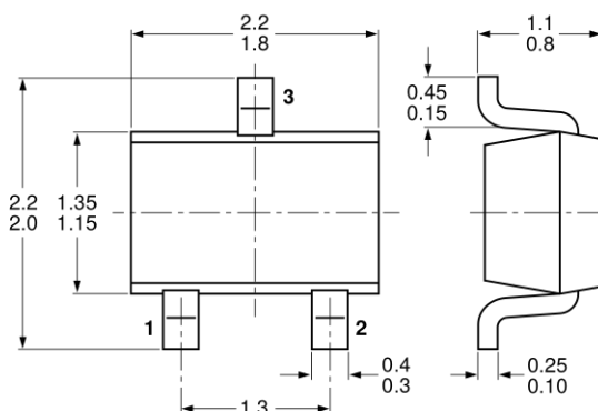
Fig 10. Package outline SOT323 (SC-70)
