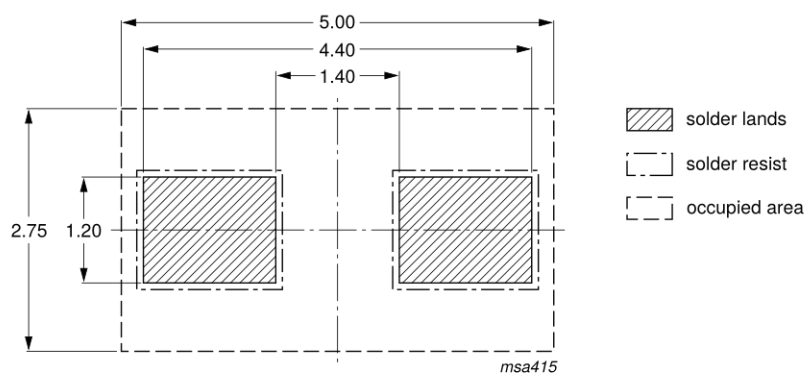
Fig 15. Reflow soldering footprint SOD323 (SC-76)
