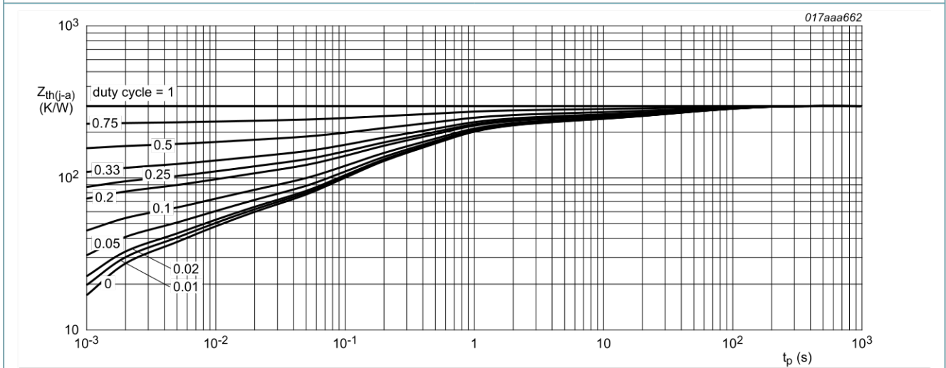
FR4 PCB, mounting pad for drain 1 cm 2
