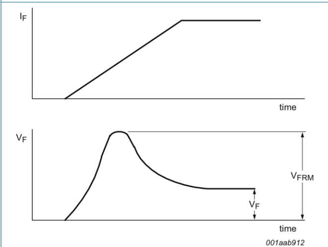
Fig. 7. Forward recovery definitions
