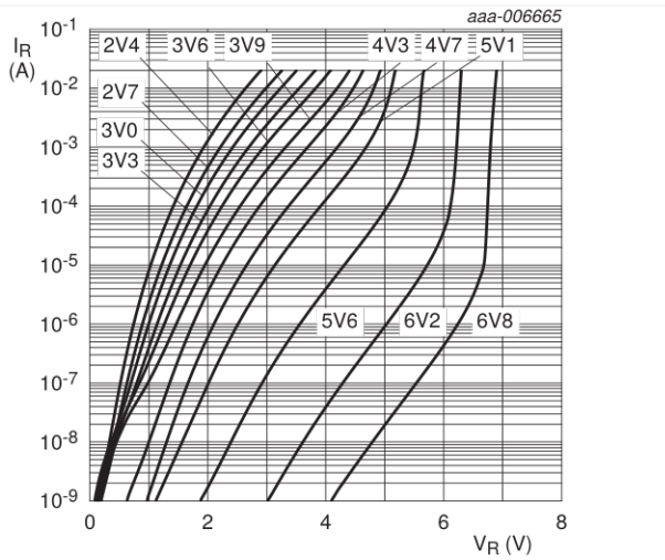
BZX84-A/B/C2V4 to BZX84-A/B/C6V8 T_{amb} = 25\text{ }^{\circ}\text{C}
