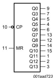
Fig. 1. Functional diagram
