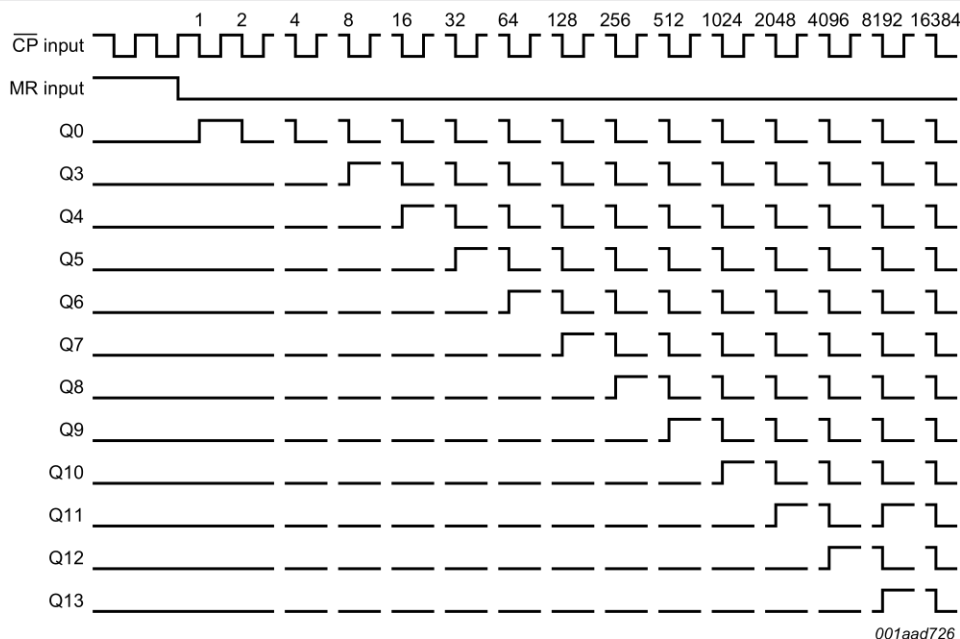
Fig. 6. Timing diagram
