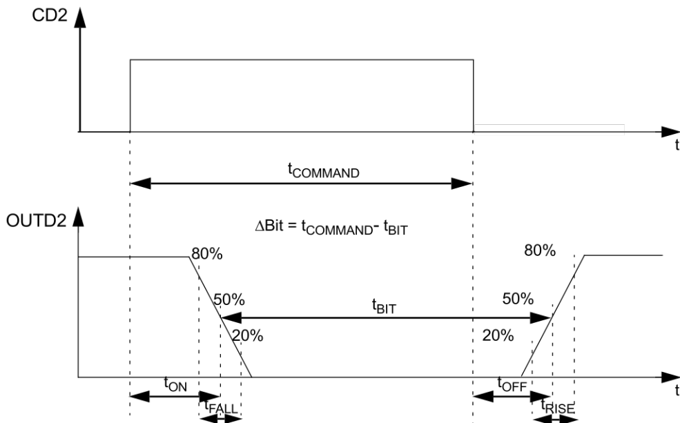
Figure 4. Timing Characteristics
