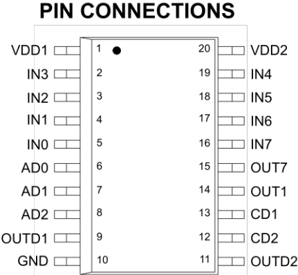
Figure 3. 33287 Pin Connections
