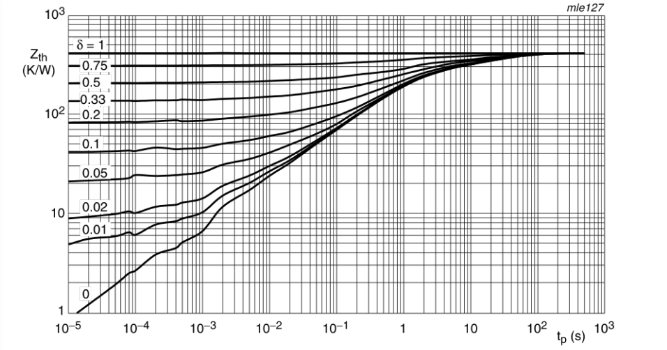
Fig 2. Transient thermal impedance as a function of pulse duration; typical values
