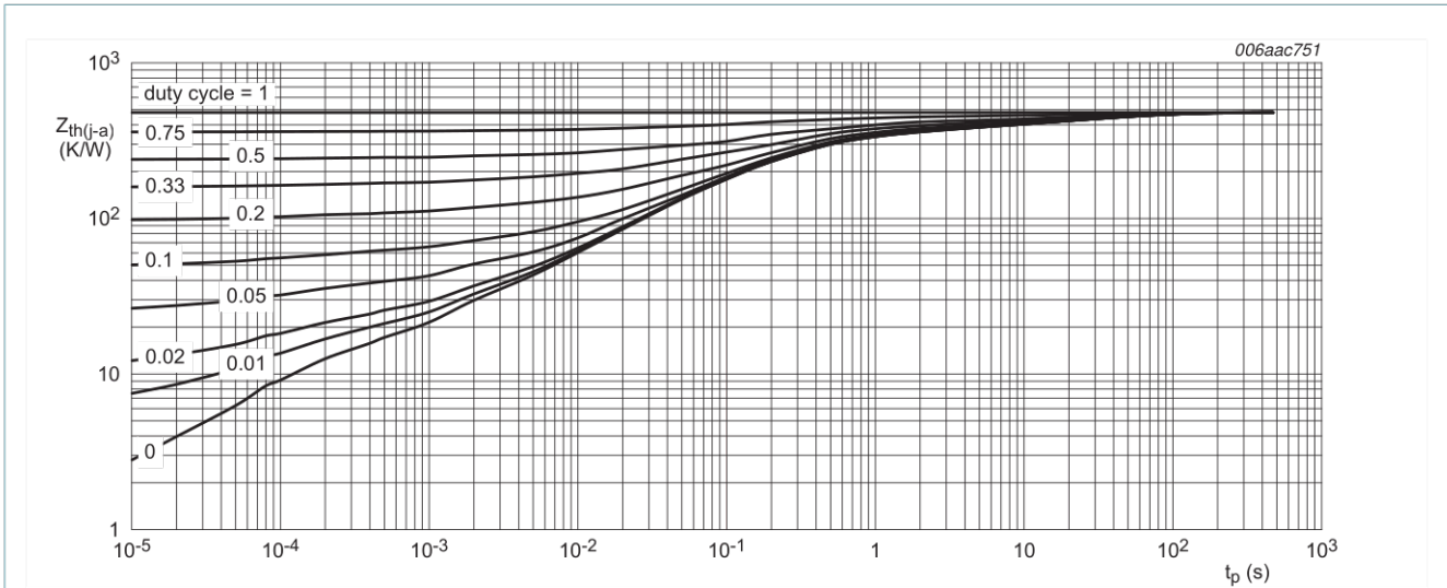
Fig 2. Per transistor: Transient thermal impedance from junction to ambient as a function of pulse duration for PEMD12 (SOT666); typical values
