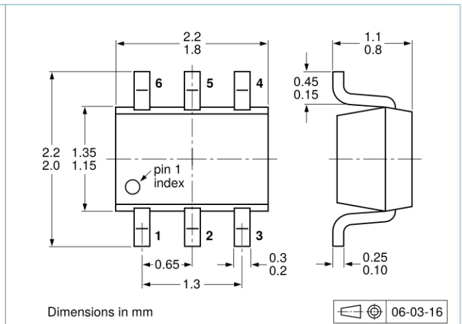
Fig 17. Package outline PUMD12 (SOT363)
