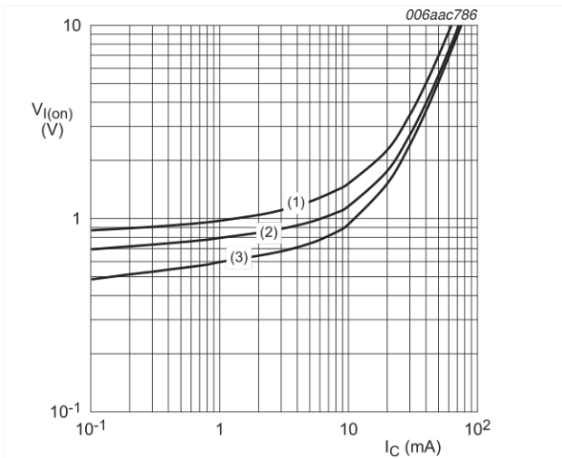
V_{CE} = 0.3\text{ V} (1) T_{amb} = -40\text{ }^{\circ}\text{C} (2) T_{amb} = 25\text{ }^{\circ}\text{C} (3) T_{amb} = 100\text{ }^{\circ}\text{C}
