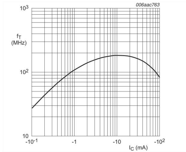
V_{CE} = -5 \text{ V}; T_{amb} = 25 \text{ }^\circ\text{C}
