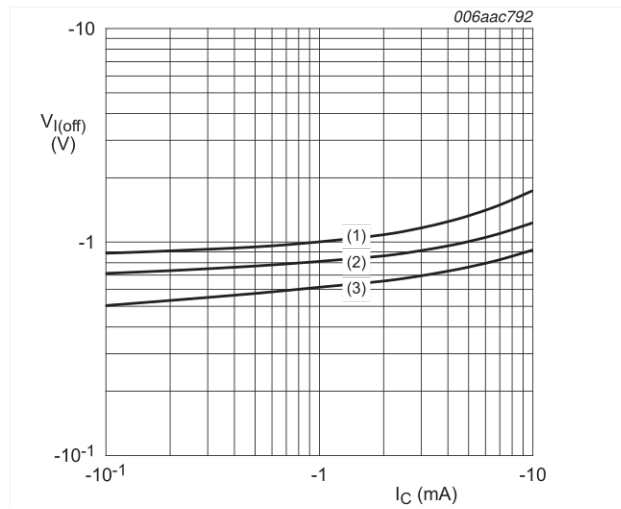
V_{CE} = -5 \text{ V} (1) T_{amb} = -40 \text{ }^\circ\text{C} (2) T_{amb} = 25 \text{ }^\circ\text{C} (3) T_{amb} = 100 \text{ }^\circ\text{C}
