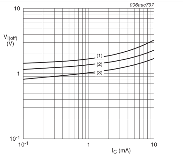
V_{CE} = 5\text{ V} (1) T_{amb} = -40\text{ }^{\circ}\text{C} (2) T_{amb} = 25\text{ }^{\circ}\text{C} (3) T_{amb} = 100\text{ }^{\circ}\text{C}
