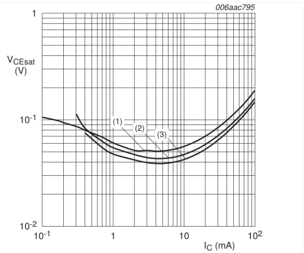
I_C/I_B = 20 (1) T_{amb} = 100\text{ }^{\circ}\text{C} (2) T_{amb} = 25\text{ }^{\circ}\text{C} (3) T_{amb} = -40\text{ }^{\circ}\text{C}
