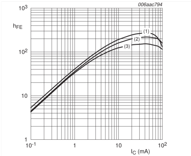
V_{CE} = 5\text{ V} (1) T_{amb} = 100\text{ }^{\circ}\text{C} (2) T_{amb} = 25\text{ }^{\circ}\text{C} (3) T_{amb} = -40\text{ }^{\circ}\text{C}
