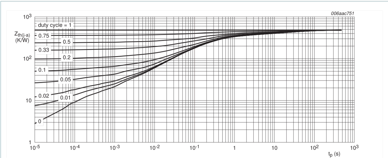
Fig 2. Per transistor: Transient thermal impedance from junction to ambient as a function of pulse duration for PEMH1 (SOT666); typical values
