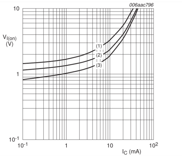
V_{CE} = 0.3\text{ V} (1) T_{amb} = -40\text{ }^{\circ}\text{C} (2) T_{amb} = 25\text{ }^{\circ}\text{C} (3) T_{amb} = 100\text{ }^{\circ}\text{C}
