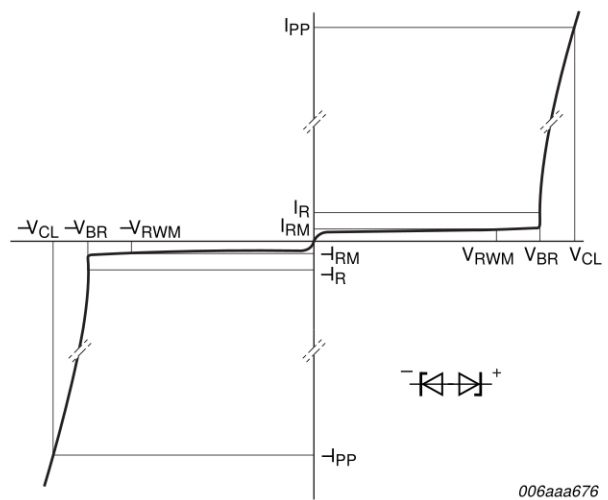
Fig 6. V-I characteristics for a bidirectional protection diode
