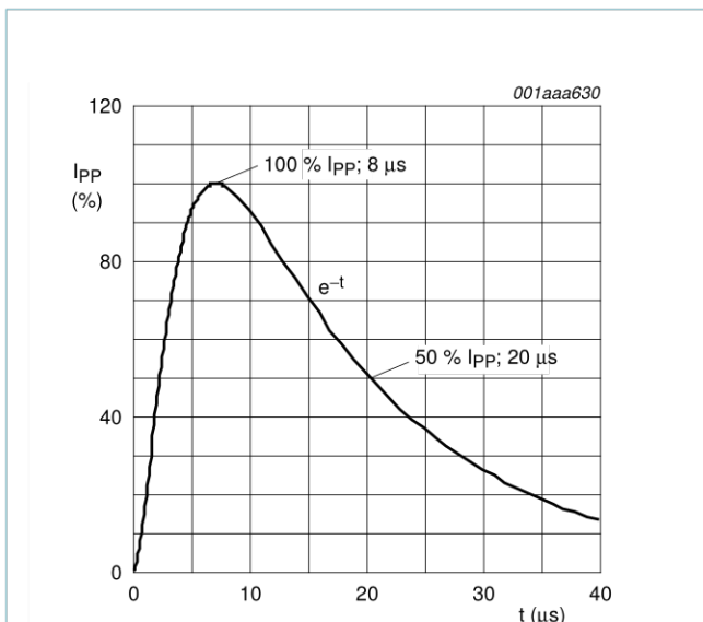
Fig 1. 8/20 μs pulse waveform according to IEC 61000-4-5
