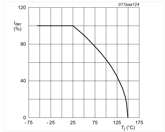
Fig. 2. MOSFET transistor: Normalized continuous drain current as a function of junction temperature
