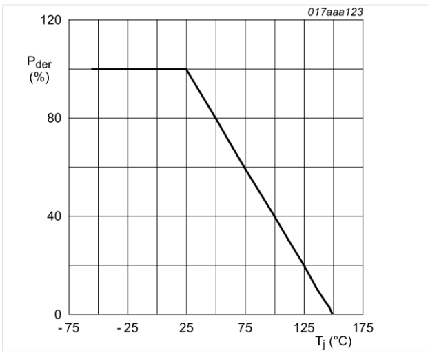
Fig. 1. MOSFET transistor: Normalized total power dissipation as a function of junction temperature
