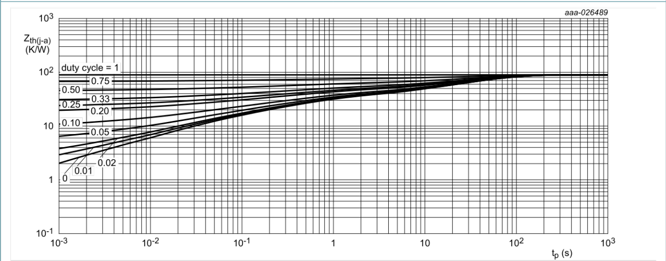
FR4 PCB, mounting pad for cathode 1 cm 2
