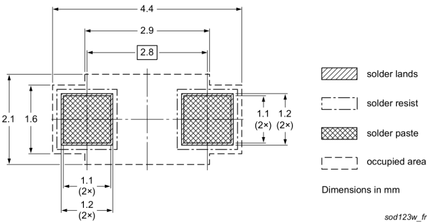
Fig. 16. Reflow soldering footprint for CFP3 (SOD123W)
