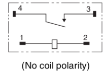
Terminal Arrangement/ Internal Connections (BOTTOM VIEW)
