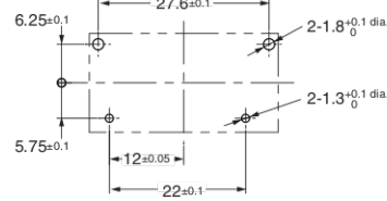
PCB Mounting Holes (BOTTOM VIEW)
