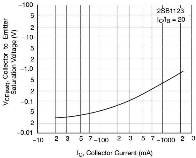
Figure 13. V_{CE(sat)} - I_C
