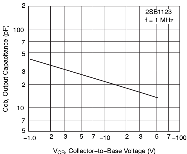
Figure 11. C_{ob} - V_{CB}
