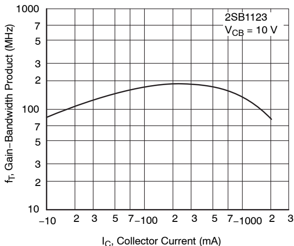
Figure 9. f_T - I_C
