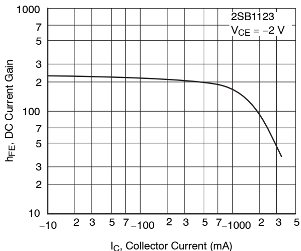
Figure 7. h_{FE} - I_C
