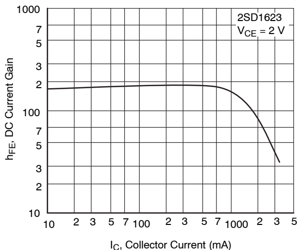
Figure 8. h_{FE} - I_C
