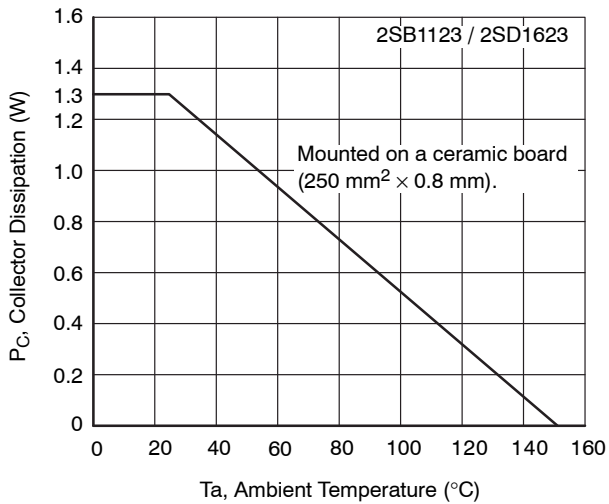
Figure 17. P_C - T_a
