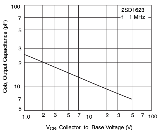
Figure 12. C_{ob} - V_{CB}
