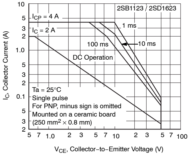
Figure 15. ASO
