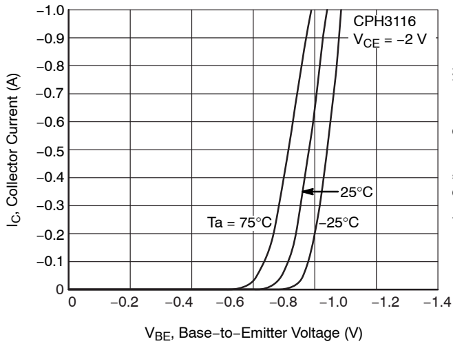
Figure 4. I_C - V_{BE}
