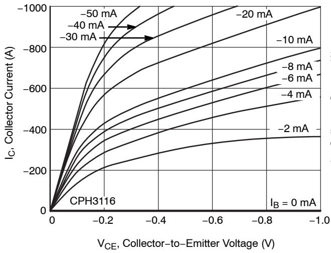
Figure 2. I_C - V_{CE}
