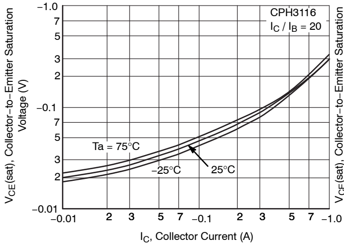
Figure 12. V_{CE(sat)} - I_C
