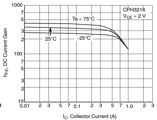
Figure 7. h_{FE} - I_C
