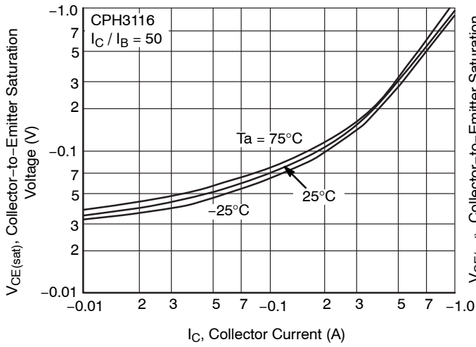
Figure 14. V_{CE(sat)} - I_C
