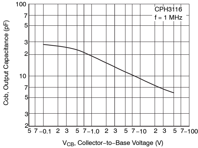
Figure 10. C_{ob} - V_{CB}
