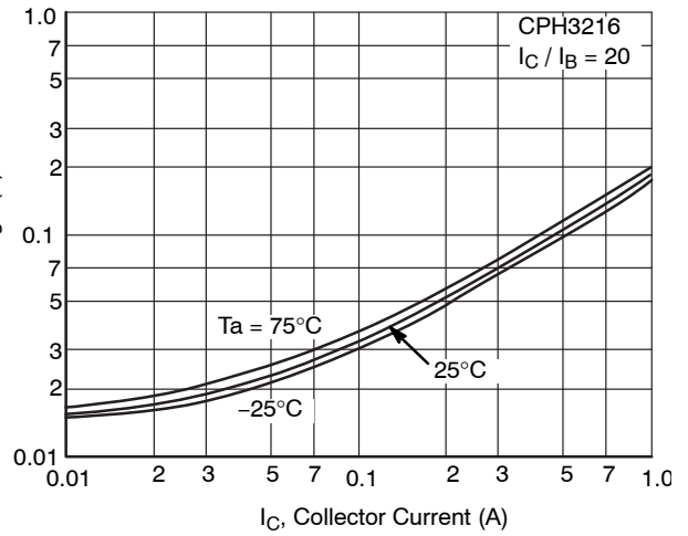
Figure 13. V_{CE(sat)} - I_C
