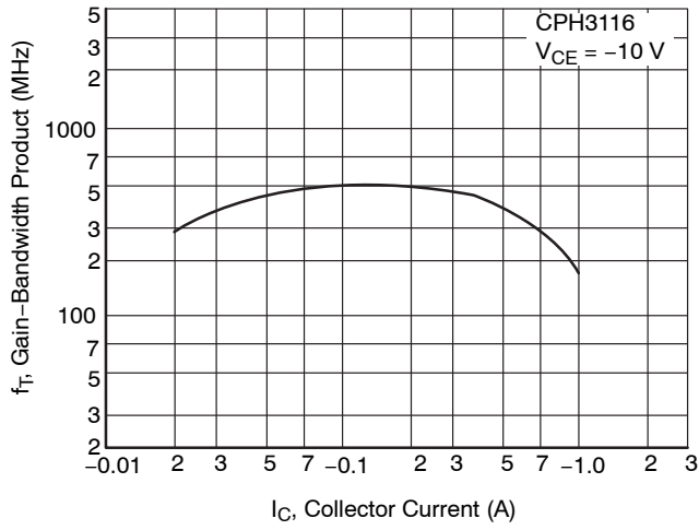
Figure 8. f_T - I_C
