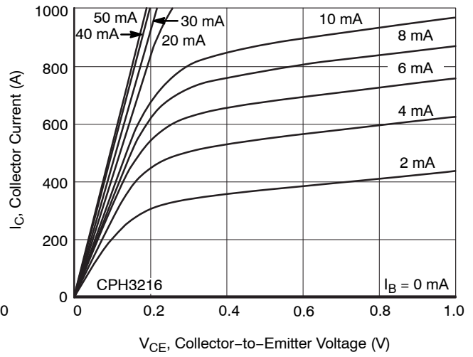
Figure 3. I_C - V_{CE}
