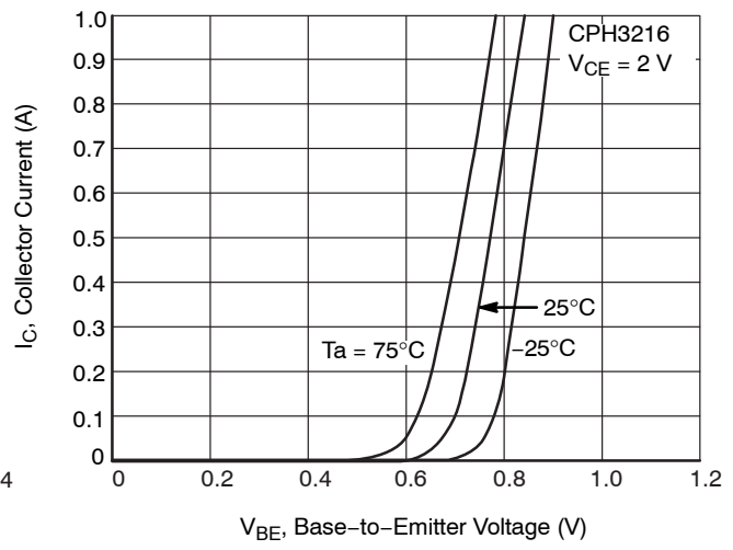
Figure 5. I_C - V_{BE}
