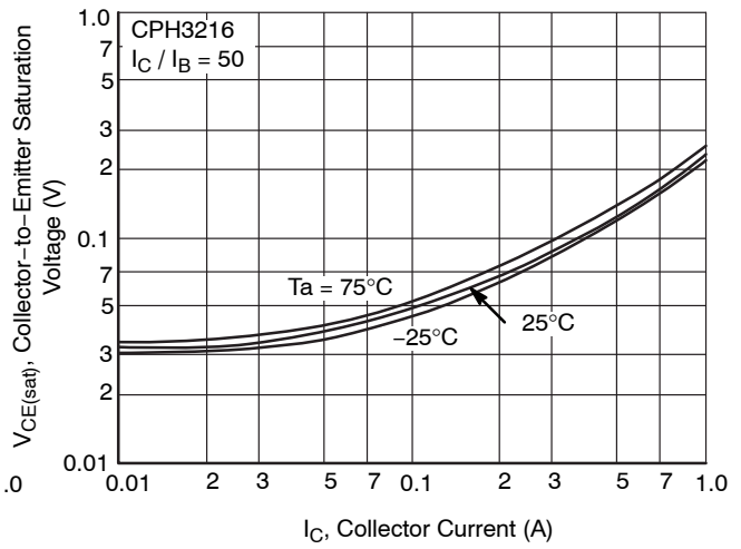
Figure 15. V_{CE(sat)} - I_C
