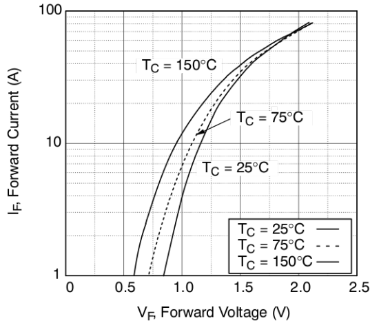
Figure 19. Forward Characteristics
