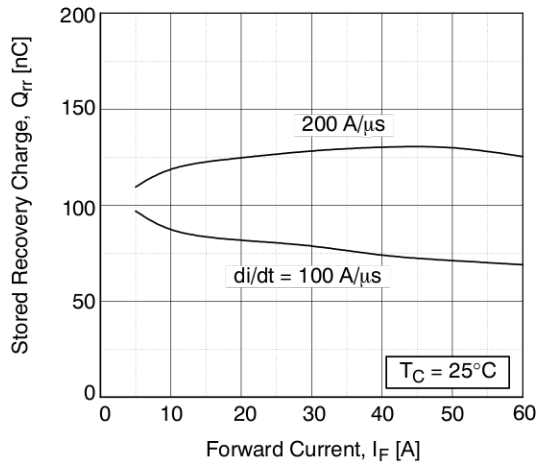
Figure 21. Stored Charge
