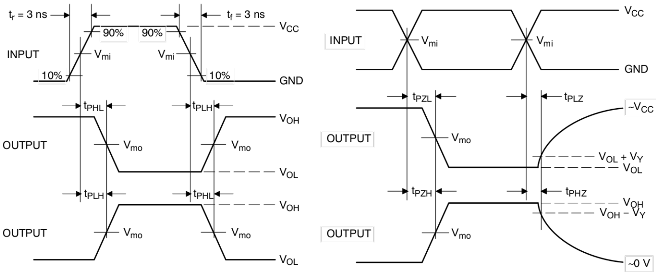
Figure 4. Switching Waveforms
